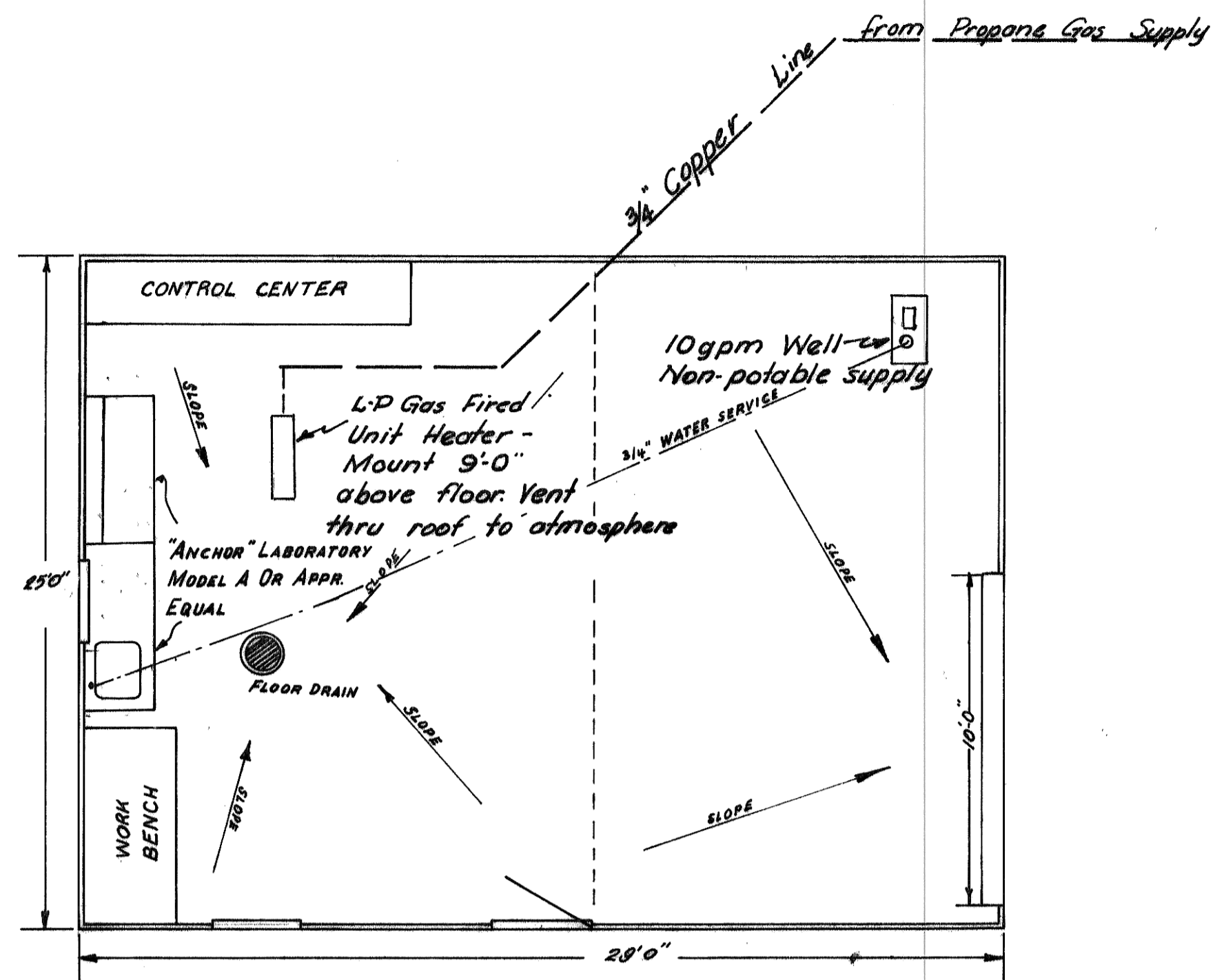
PLAN VIEW SCALE: 1/4" = 1'
