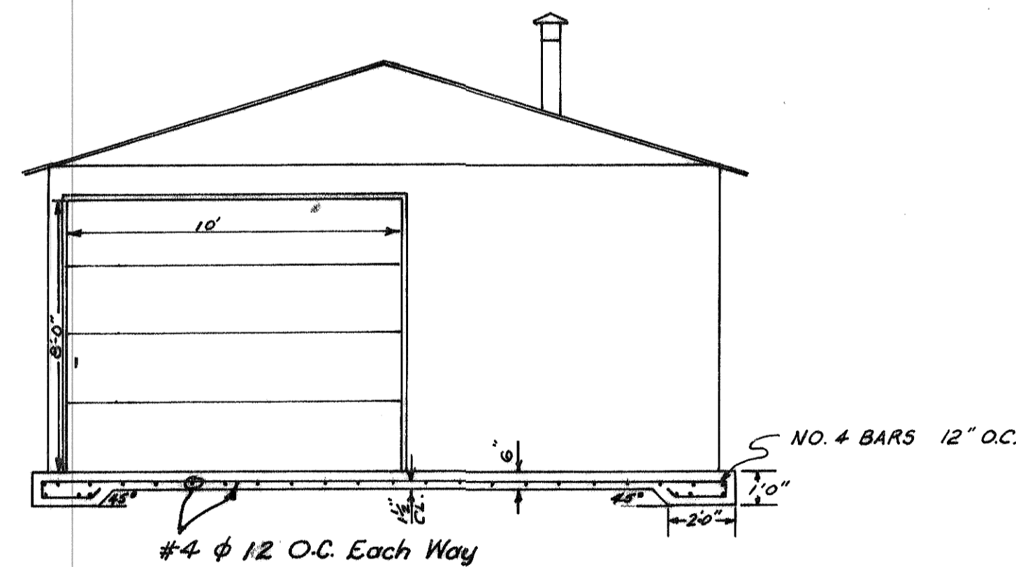
NORTH ELEVATION SCALE: 1/4" = 1'
