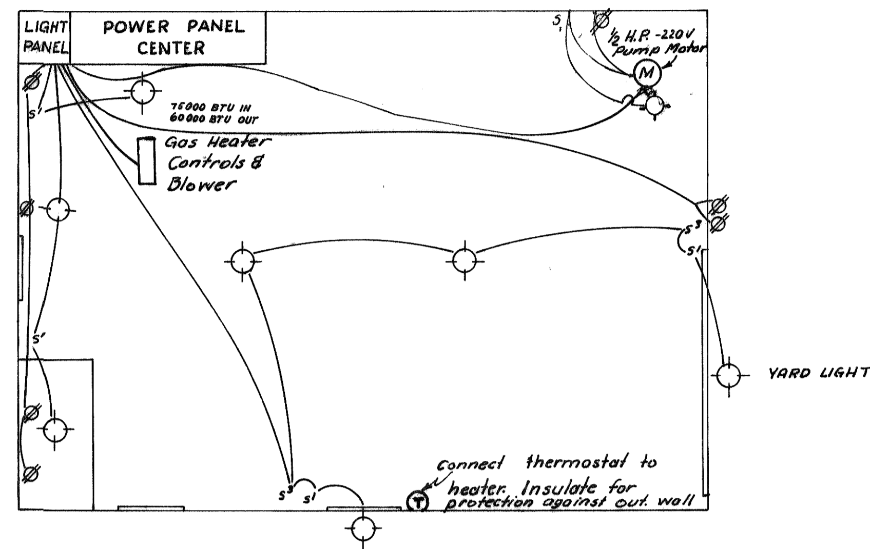
BLDG LIGHTING LAYOUT SCALE: 1/4" = 1'
